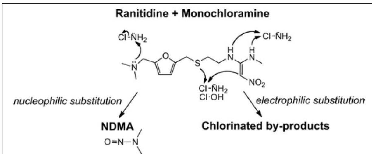
Figure 2 –Mechanism for Decomposition of Ranitidine in NDMA
